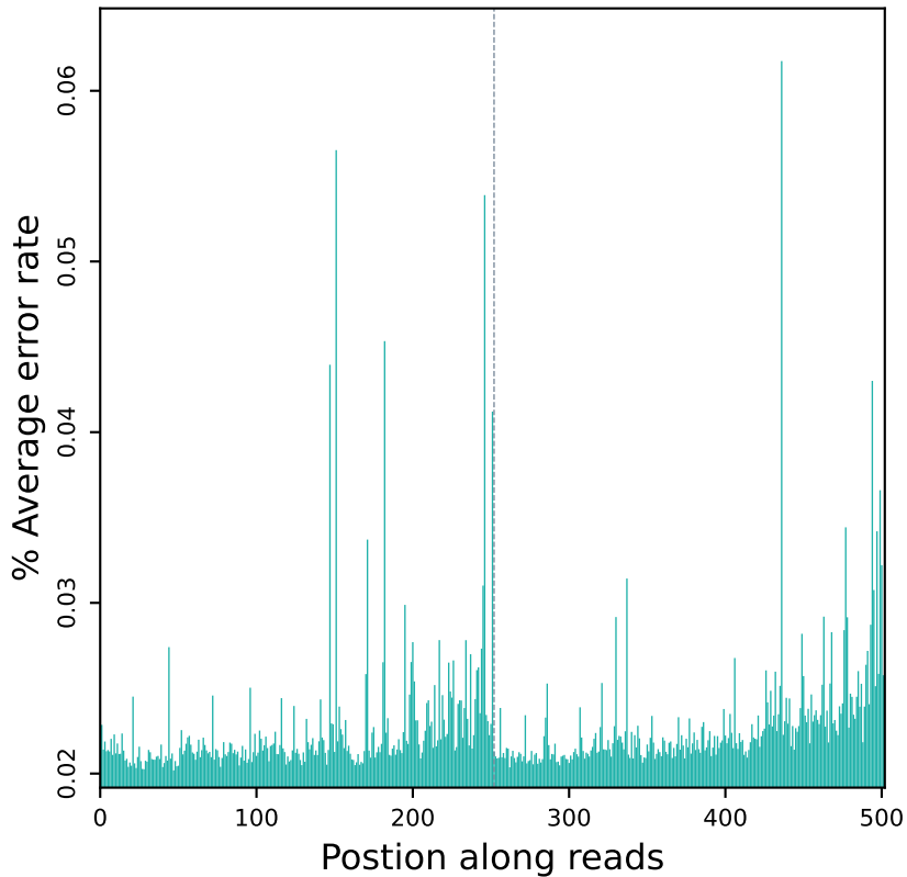
Error rate distribution along reads (R10912)
